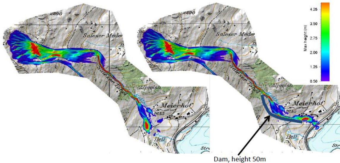
Figure 4-25: Simulation without (left) and with (right) a dam.
