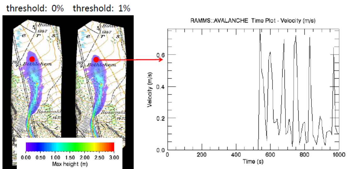
Figure 4-19: Stopping behaviour of a RAMMS simulation. Small threshold values may lead to unlikely slow
