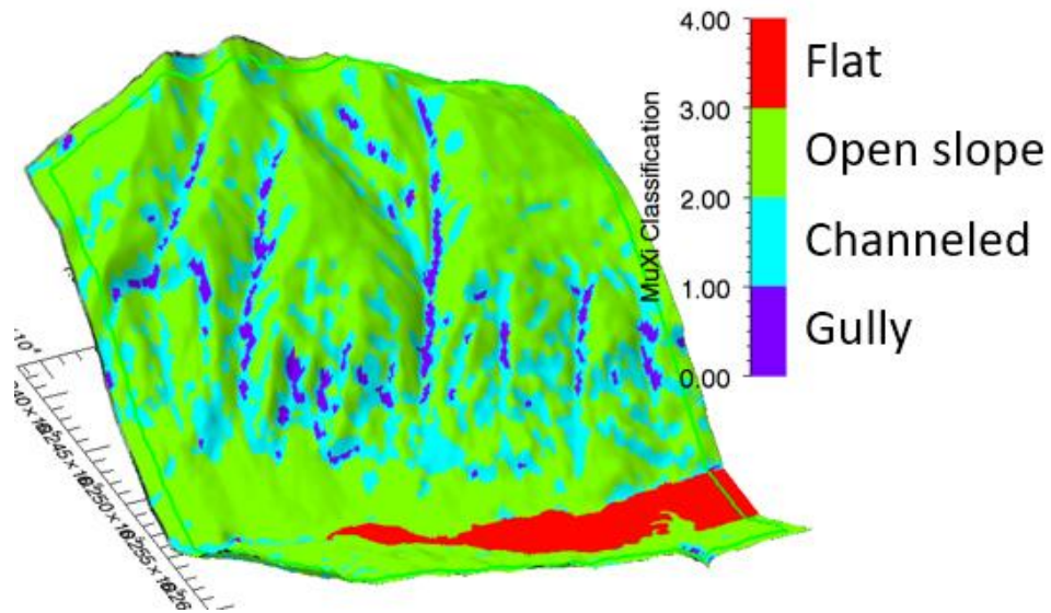
Figure 3-5: Automatic terrain analysis in RAMMS
