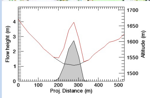
Figure 4-9: Line profile perpendicular to flow direction.
